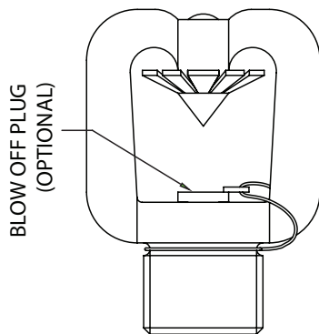
Nozzle with Blow-off Plug
